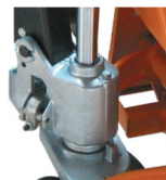
One Piece Cast Iron Pump features high quality seals, hardened and chrome-plate ram and piston, top-of-stroke and overload bypass valves
